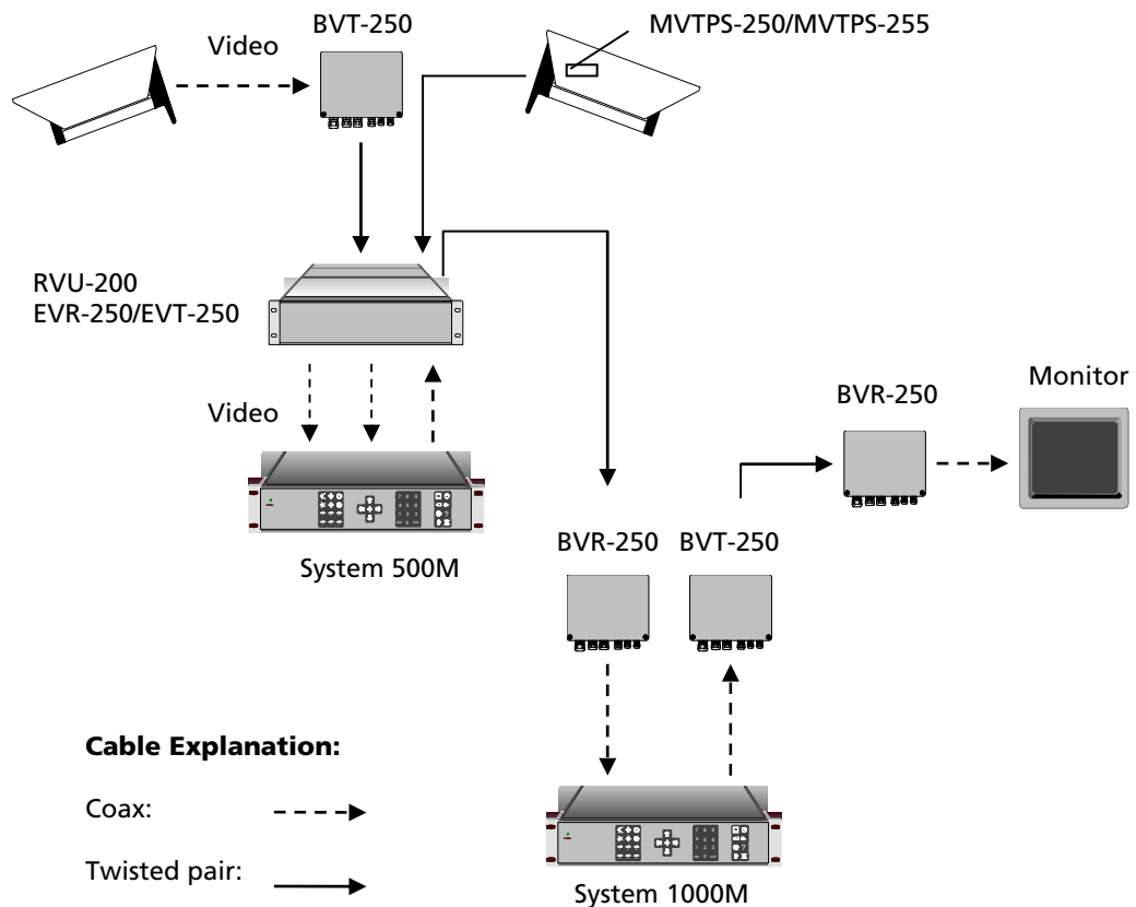
Application diagram for the Fibre Series 250
